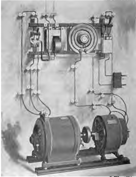
FIG. 320.—Waverley Motor-generator Charging Set for Use on a Single-phase Alternating Current Circuit of 100 to 110 Volts (60 Cycles). This apparatus will give a current of 15 amperes at 65 volts in charging a 24-cell battery, or 10 amperes in charging a 30-cell battery.
